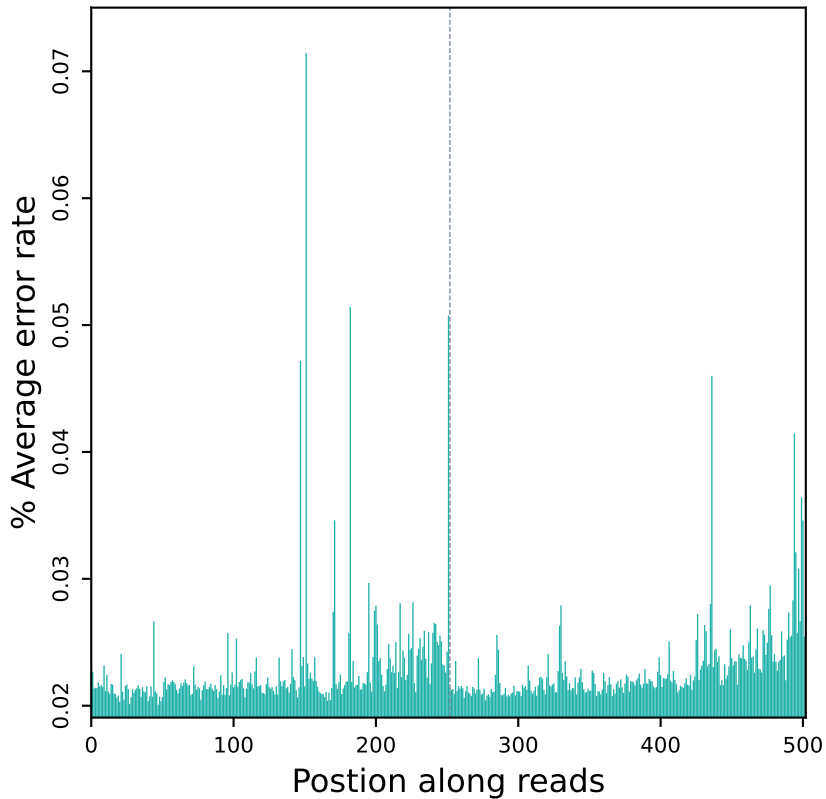
Error rate distribution along reads (R10911)
